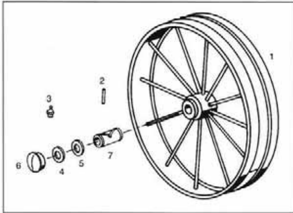
Model 350-C (Post-1982) Pop-On Hubcap
