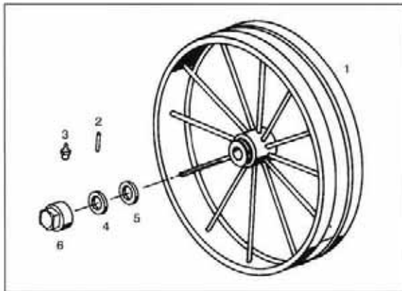
Model 350-D and 33-D (1980-1982) Threaded Hubcap
