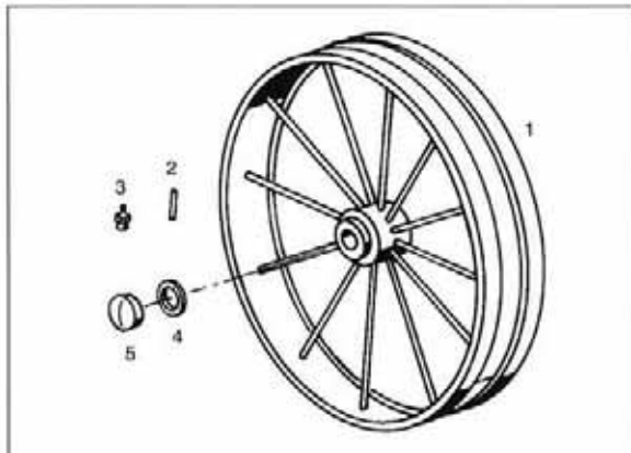
Model 350-D and 33-D (Post-1982) Pop-On Hubcap
