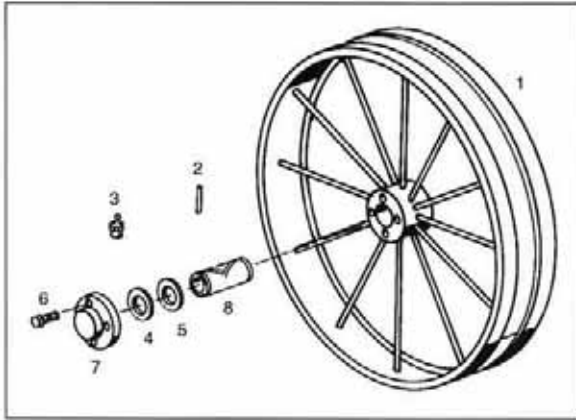
Model 350-A/B/C (Pre-1982) 4-Hole Bolt-On Hubcap
